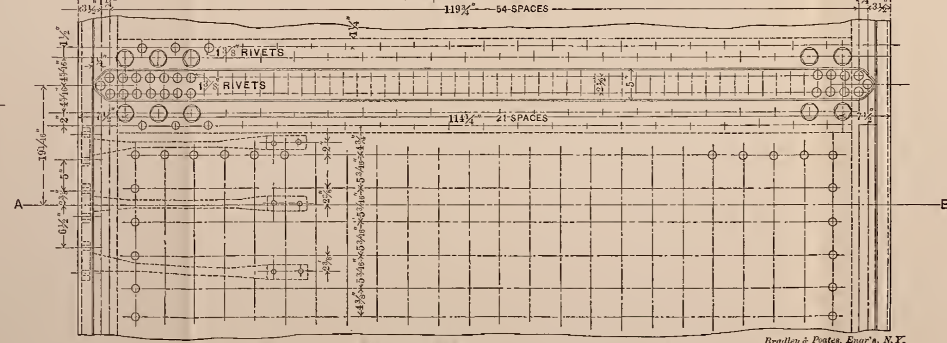
LONGITUDINAL SEAM ON OUTSIDE OF FIRE BOX
